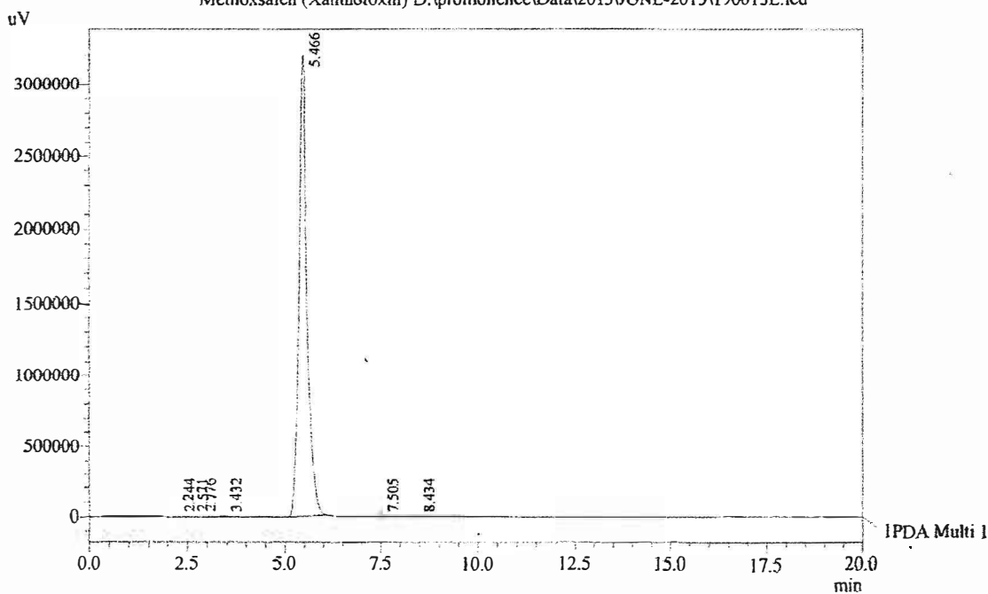
Chromatogram Methoxsalen (Xanthotoxin) D:\promonence\Data\2013\JUNE-2013\190613E.lcd
